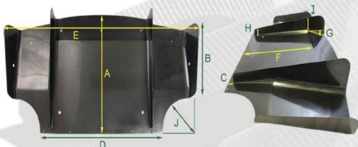
111R STAGE 2 5 rear centre tunnel fixing holes and 3 side fixing holes
