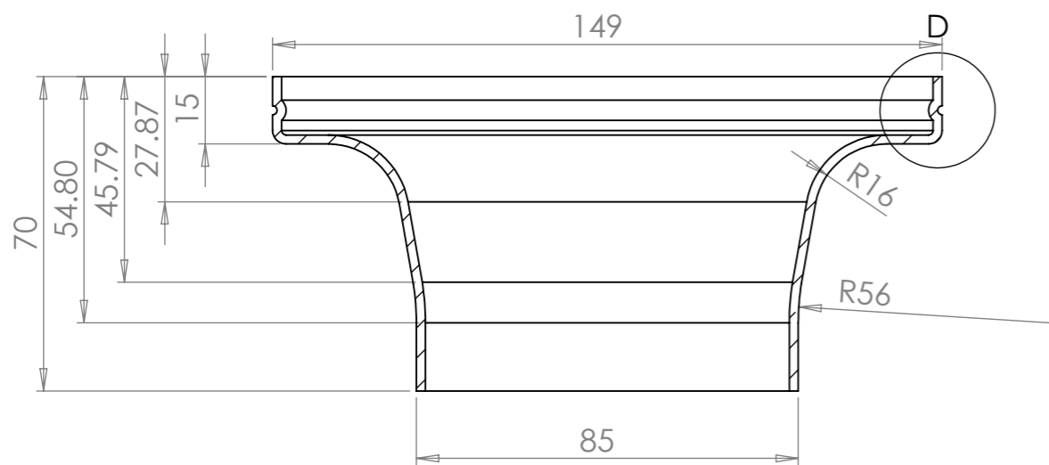
SECTION C-C SCALE 1 : 1.5
