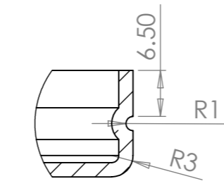
DETAIL D SCALE 2 : 1.5
